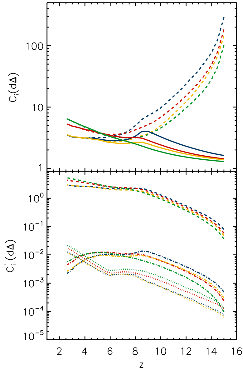
Figure 4.11: Redshift evolution of the clumping factor C_i(d\Delta) (top panel) and C'_i(d\Delta) (bottom panel) for i = \text{gas} (solid line), HII (dashed line), HeII (dot dashed line) and HeIII (dotted line). In both panels, d\Delta = 0.1 - 100 . The simulations used in these plots are 2.20G128 (blue, default), 4.39G128 (red), 8.78G128 (green) and 2.20G64 (yellow).
