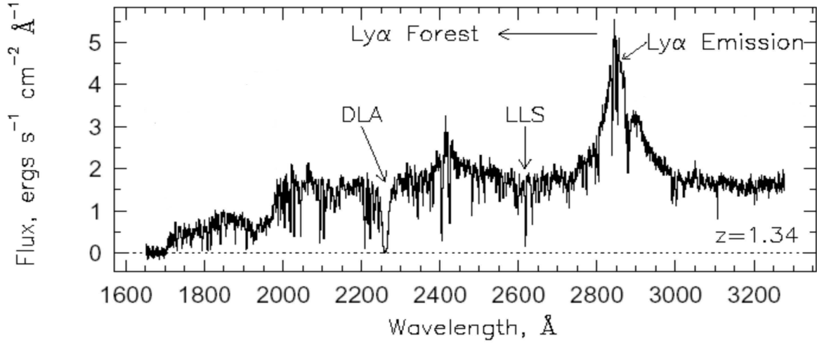
Figure 1.4: The typical spectra of a QSO at z = 1.34 with the \text{Ly}\alpha emission and absorption lines. From http://www.hs.uni-hamburg.de/EN/For/Exg/Igm/index.html .
