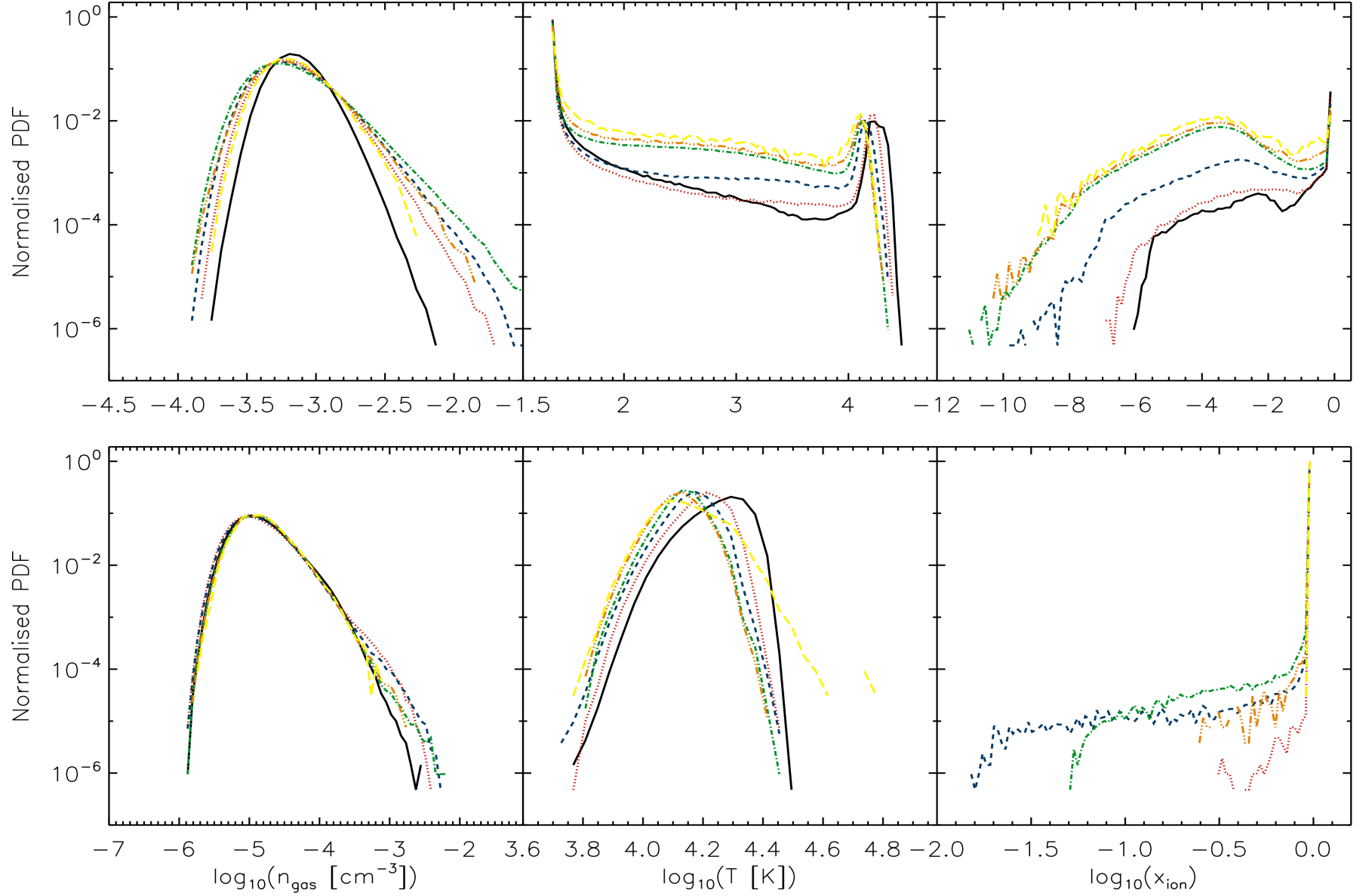
Figure 4.2: Normalized PDF of gas number density (left column), temperature (middle column) and hydrogen ionization fraction (right column) in simulations at redshifts z = 14.5 (top row) and z = 3.8 (bottom row). The lines are for -35.12G128 (black solid line), 8.78G128 (red dotted line), 4.39G128 (blue dashed line), 2.20G128 (green dot dashed line), 2.20G64 (orange triple dot dashed line) and 2.20G32 (yellow long dashed line).
