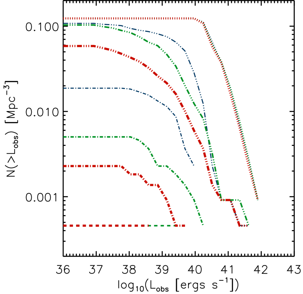
Figure 3.20: Luminosity functions calculated for the 45 most massive objects in L05 for different surface brightness cuts. The runs are for initial volume averaged ionization fraction x_{\text{ion}}=0 (red), x_{\text{ion}} = 0.5 (green) and x_{\text{ion}} = 0.89 (blue). The SB thresholds are SB_{\text{th}} = 10^{-25} (dotted lines), 10^{-21} (triple dot dashed lines), 10^{-20} (dot dashed lines) and 5 \times 10^{-20} (dashed lines) \text{ergs s}^{-1} \text{ cm}^{-2} \text{ arcsec}^{-2} .
