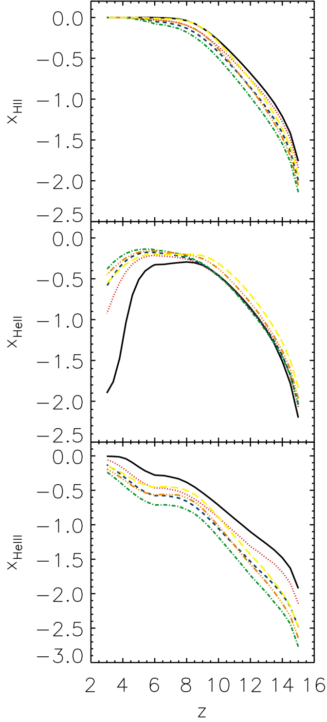
Figure 4.5: Redshift evolution of the volume averaged ionization fractions - x_{\text{HII}} (upper panel), x_{\text{HeII}} (middle) and x_{\text{HeIII}} (lower) for the 35.12G128 (black solid line), 8.78G128 (red dotted), 4.39G128 (blue dashed), 2.20G128 (green dot-dashed), 2.20G64 (orange triple dot-dashed) and 2.20G32 (yellow long-dashed) runs.
