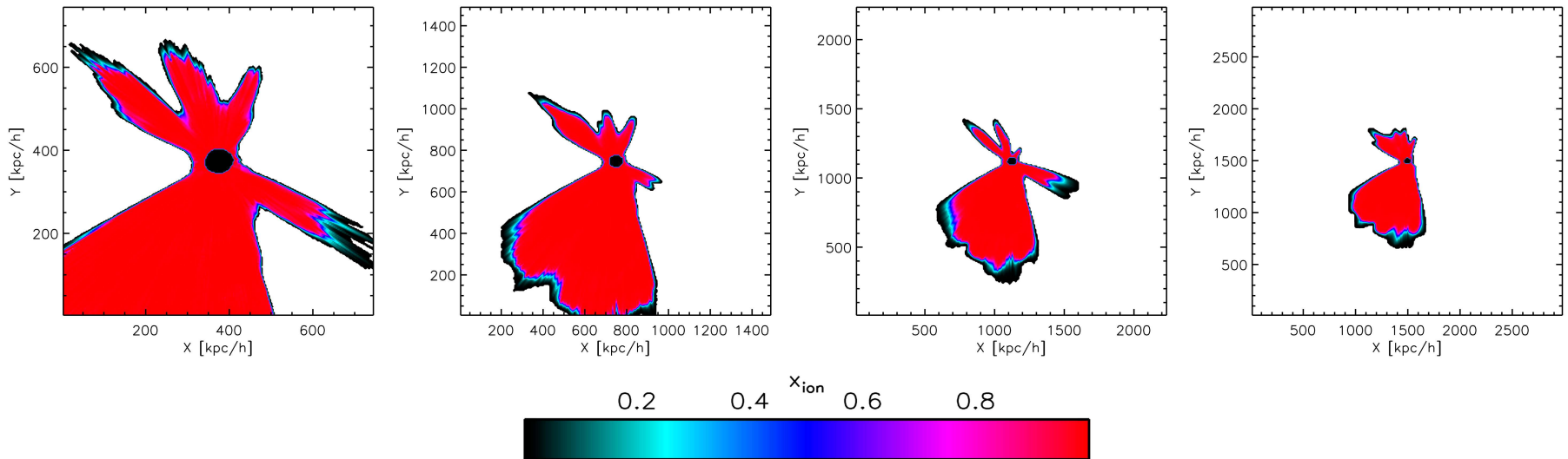
Figure B.1: A slice through the ionization structure in the cube for simulations with different cube sizes of the IGM around the source. The degree of ionization of the gas is shown by the color bar at the bottom. The panels are for simulations of different cube sizes - \sim 12 r_{200} (left panel), \sim 23 r_{200} (centre left panel), \sim 35 r_{200} (centre right panel), \sim 47 r_{200} (right panel) where r_{200} is the radius in comoving units at which the mean DM density inside the sphere is 200 times the critical density of the universe at that redshift.
