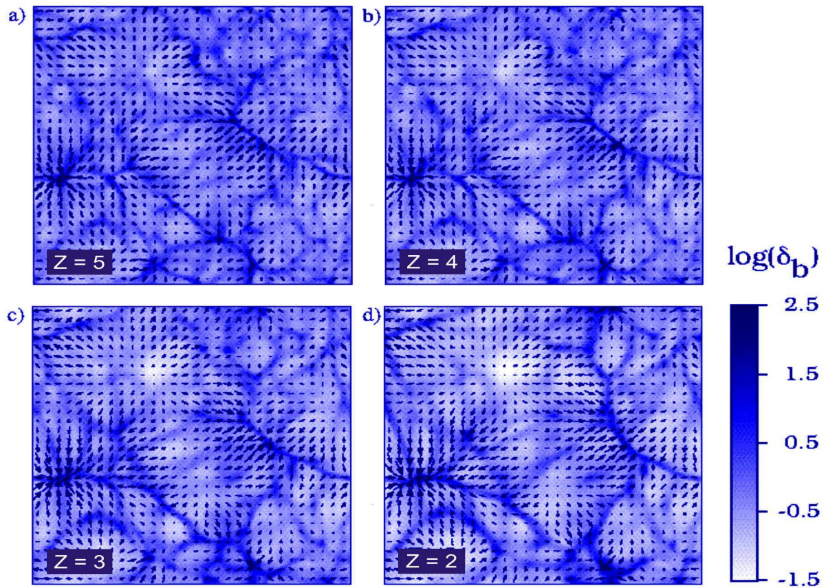
Figure 1.3: From Zhang et al. (1998) - The evolution of baryon overdensity distribution. The baryon overdensities in the box are shown at z = 2, 3, 4 , and 5 . Superimposed as arrows is the peculiar velocity field.
