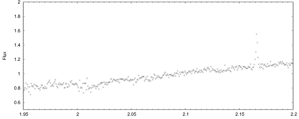
Figure 6.4: Total flux of MWC 14 over total flux of the calibrator versus wavelength as obtained with AMBER. No molecular lines can be identified, but one can clearly see the Br \gamma line at 2.166 \mu\text{m} .
