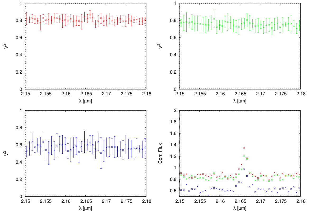
Figure 6.5: Visibilities and correlated spectra for MWC 147 as obtained with AMBER. Upper Left : Baseline UT1-UT2 (54.5 m, 35.8°) Upper right : Baseline UT2-UT3 (46.4 m, 46.2°) Lower Left : Baseline UT1-UT3 (100.4 m, 40.5918°) Lower Right : Spectrum including the Br \gamma line at 2.166 \mu\text{m} .
