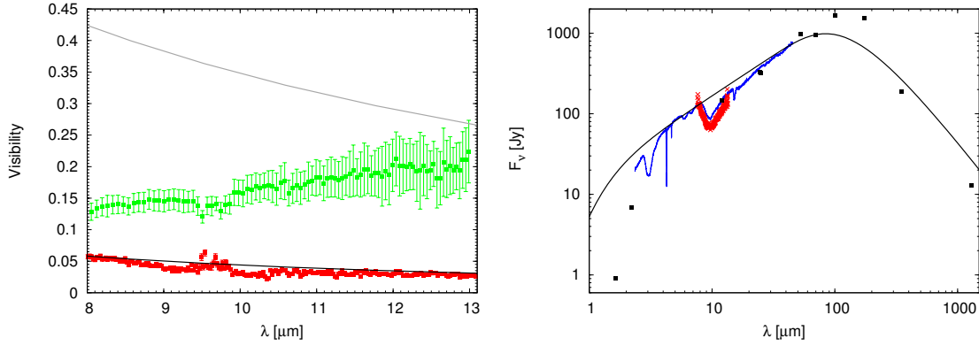
Figure 3.4: Left: Comparison of the best-fit temperature-gradient model to the visibilities of NGC 2264 IRS 1 with the model parameters described in Sect. 3.3.2 (green for the 40 m baseline, red for the 90 m baseline). The resulting modeled visibility for the 40 m baseline is shown by the gray line, the one for the 90 m baseline by the black line. Right: Comparison of the SED of our best-fit temperature-gradient model (black line) described in Sect. 3.3.2 with the ISO spectrum (blue line) of NGC 2264 IRS 1. The MIDI spectrum is shown with red crosses, all other measurements from Table 3.1 are shown with black rectangulars.
