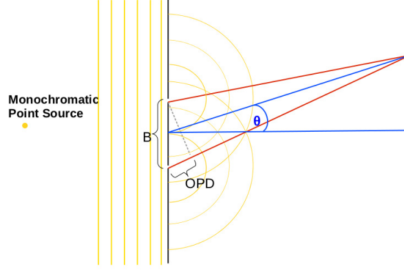
Figure 2.1: Scheme of Young's double-slit experiment. B denotes the distance of the two slits (or two telescopes).
