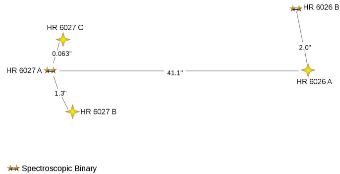
Figure 4.4: Schematic view of the \nu Sco system (not to scale)
